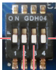
BOOT_MODE1=0 Dip Switch Configuration = 0000
