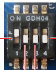
BOOT_MODE1=1 Dip Switch Configuration = 0001
